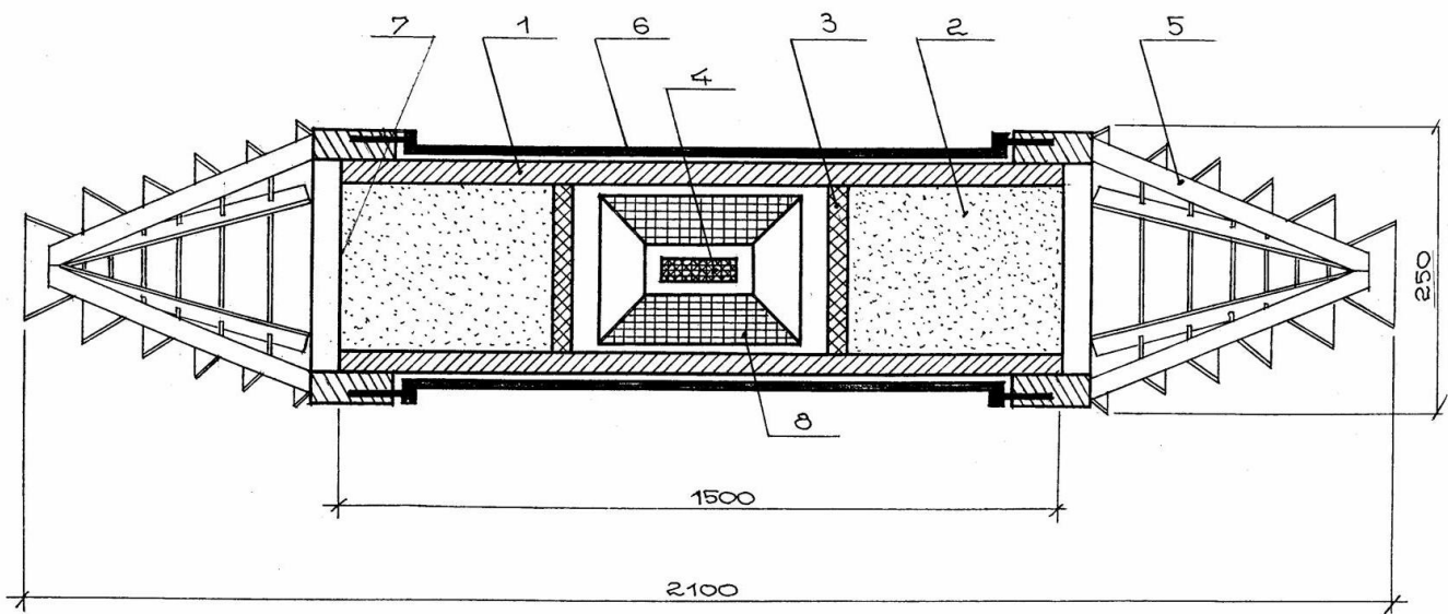
Fig. 8. - Automatic double-action explosion suppressor:
