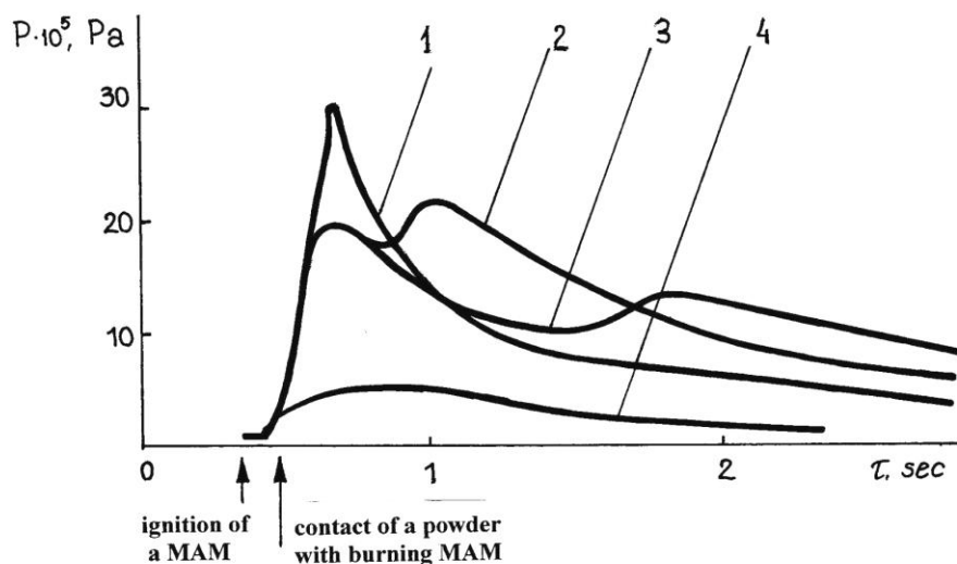
Fig. 5 - Suppression of the developed methane-air mixture explosion (MAM) by "PSE"-powder in a laboratory tube: 1- pure MAM; PSE concentration in MAM: 2 - 290 \text{ g/m}^3 ; 3 - 330 \text{ g/m}^3 ; 4- 420 \text{ g/m}^3 (explosion is suppressed)
