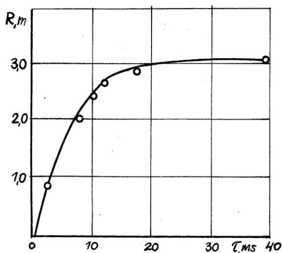
Fig. 6 - Dynamics of increase of the KCl "aerosol cloud" radius vs time during its dispersal by mini-explosion
