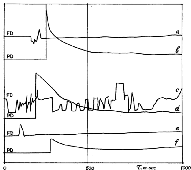
Fig. 7. - Oscillogram of the methane-air mixture (MAM) and coal dust
