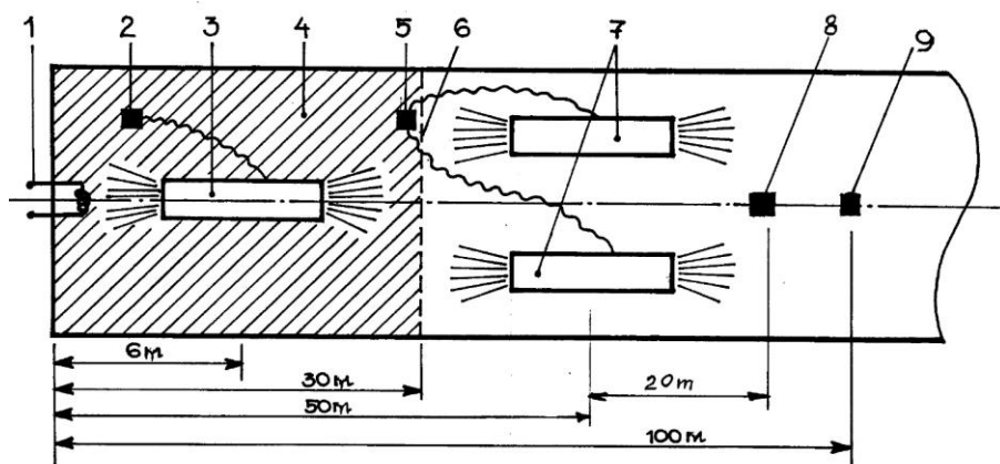
Fig. 3 - The schema of testing in the experimental edit (tunnel)
