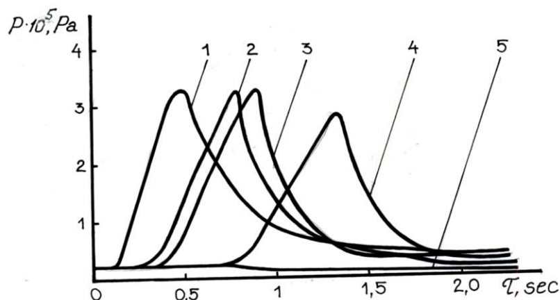
Fig. 4 - Explosion prevention of a methane-air mixture (MAM) by "PSE"-powder at the initial stage in a laboratory tube: 1- pure MAM; PSE concentrations in MAM: 2- 2.9 \text{ g/m}^3 ; 3- 5.6 \text{ g/m}^3 ; 4- 8.5 \text{ g/m}^3 ; 5- 10.1 \text{ g/m}^3 (explosion is prevented at the initial stage)
