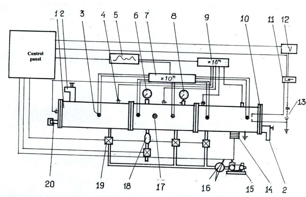
Fig. 1 - Laboratory installation for the research of explosion-suppression efficiency using powders
