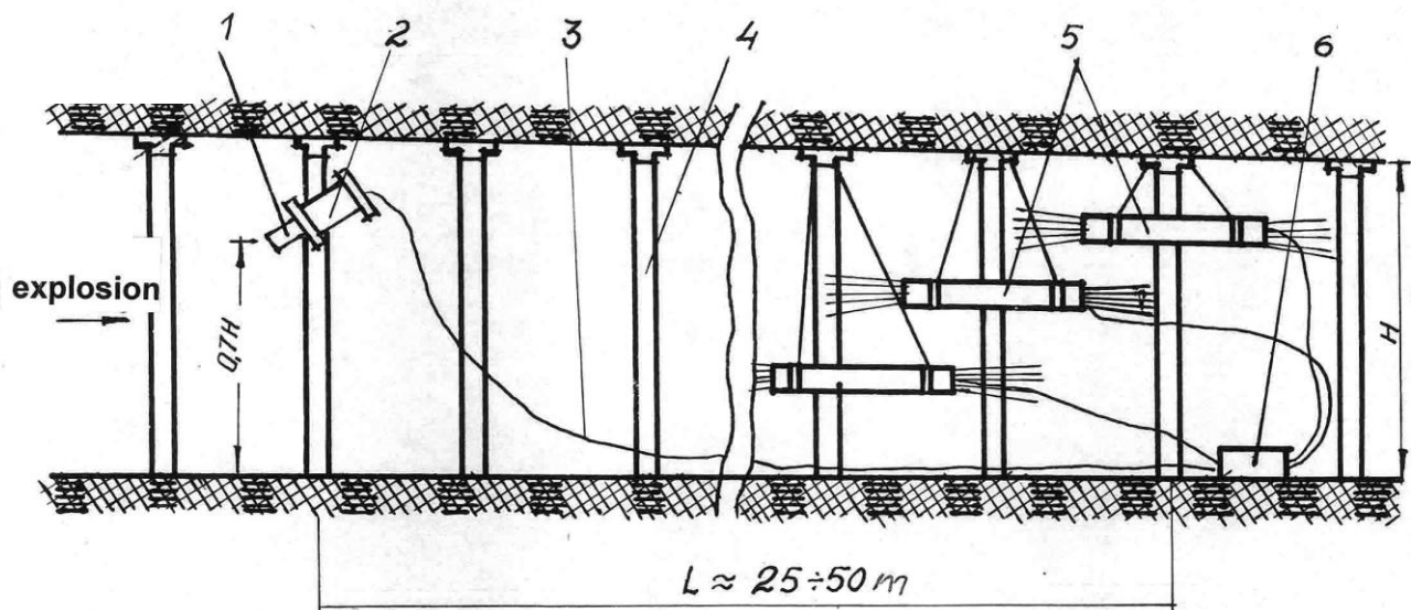
Fig. 10 - Automatic system for the suppression of explosions using PSE-powder: 1 - explosion-detector; 2 - metallic safety; 3 - communication cable; 4 - adit column; 5 - suppressors; 6 - electronics.
