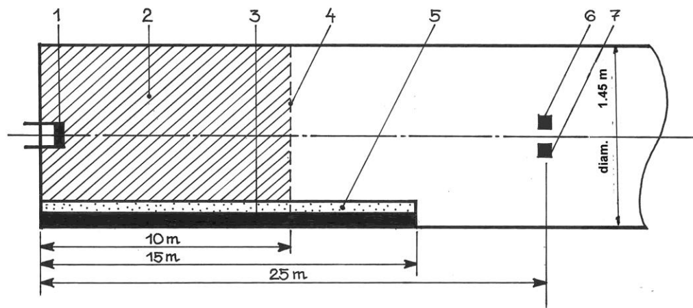
Fig. 2 - The schema of testing in the experimental tube
