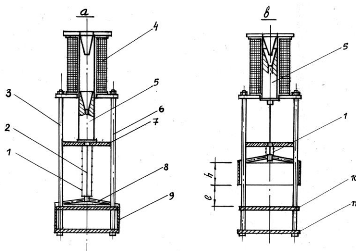
Fig. 4 - The apparatus for automatic withdrawal of aerosol samples
