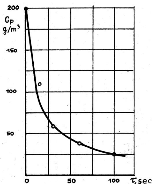
Fig. 8. Dynamics of precipitation of ammonium phosphate particles (d = 5 microns) in the 100 m 3 chamber
