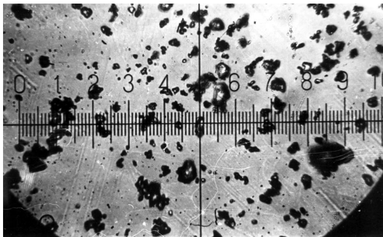
Fig. 5. Photography of a particles of factory-made ammonium phosphate powder taken in an optical microscope at 945× magnification
