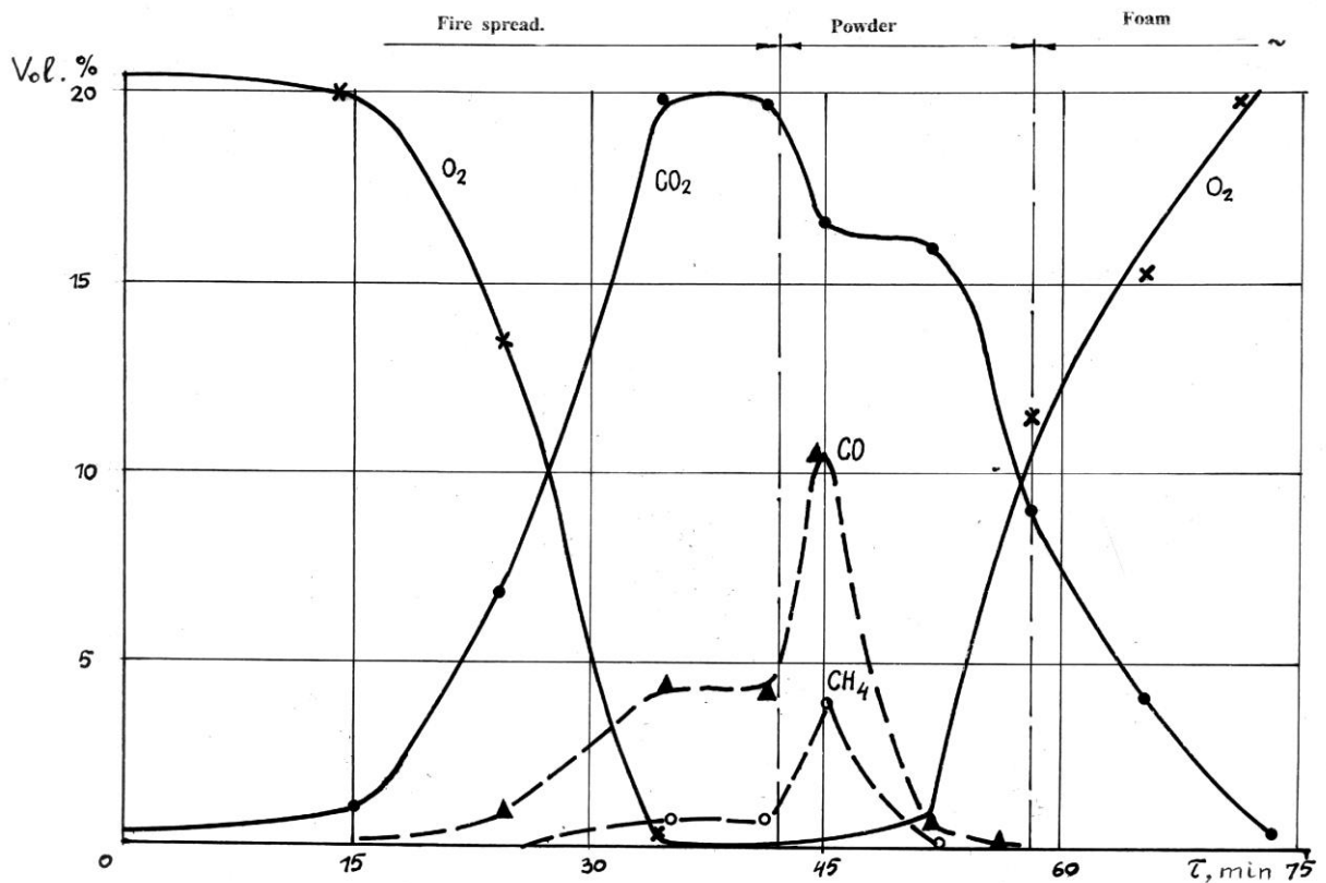
Fig. 12. Dynamics of change of fire gas composition during the extinguishing the burning timber support
