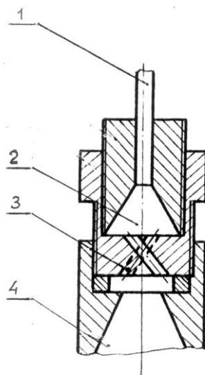
Fig. 2. The sprayer for powder aerosol
