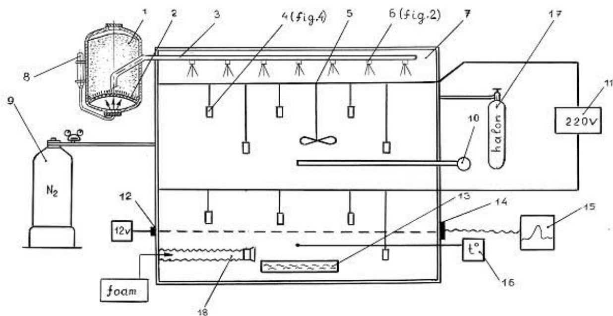
Fig. 1. Chamber used for measurement of aerosol properties
