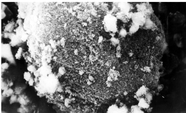
Fig. 7. Photography of surface of a conglomerate [\text{NH}_4\text{H}_2\text{PO}_4] - [\text{SiO}_2 - \text{CH}_3] in the electronic microscope at 1800× magnification
