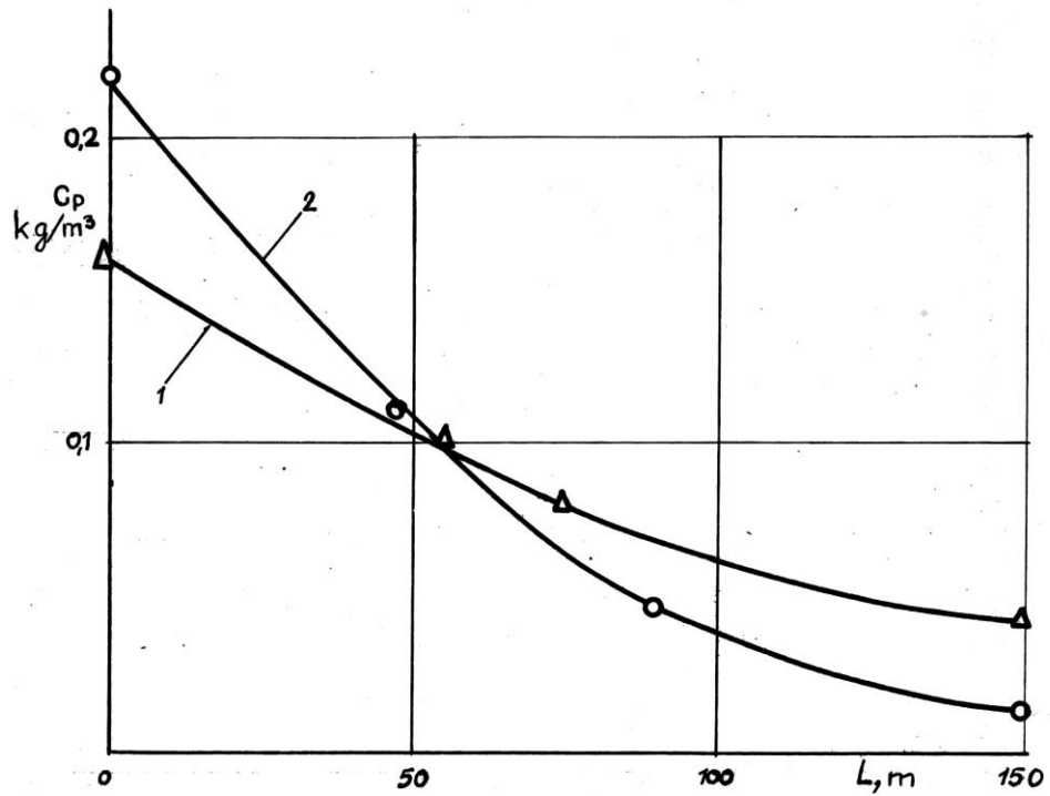
Fig. 10. Relationship between concentration ( C_p , \text{kg/m}^3 ) of powder in concurrent air stream and distance from the fire-fighting installation 1 - ammonium phosphate (diam. = 5 microns); 2 - ammonium phosphate (diam. = 40 micron).
