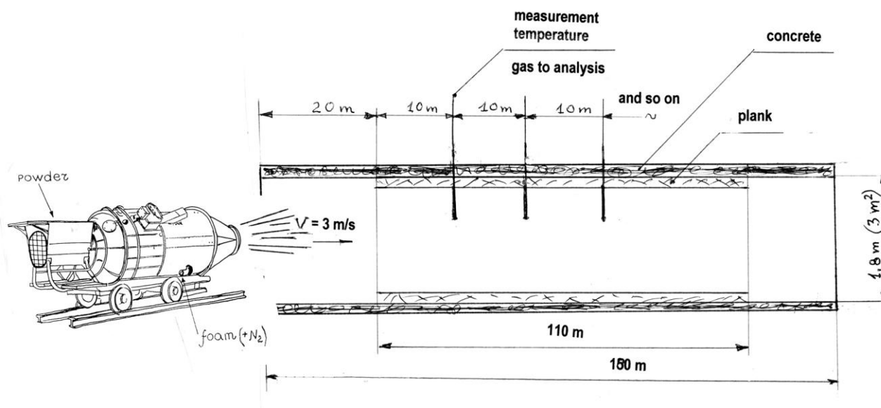
Fig. 3. Scheme of tests carried out in the experimental tunnel
